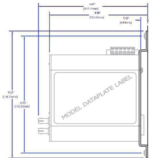
OPTIONAL COMPACT PANEL MOUNT ASSY. ( P/N: CPMA-1 )
